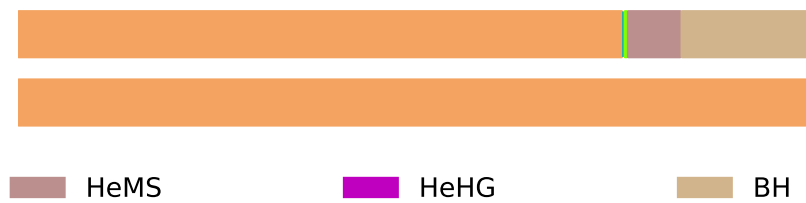
Stellar Type
