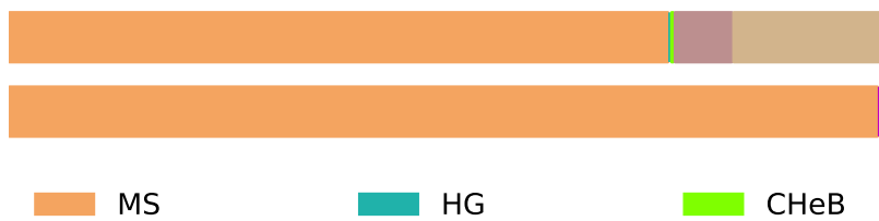
Stellar Type
