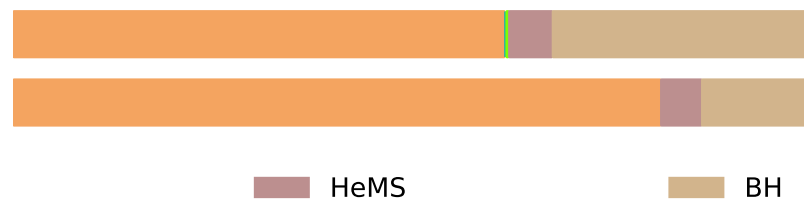
Stellar Type
